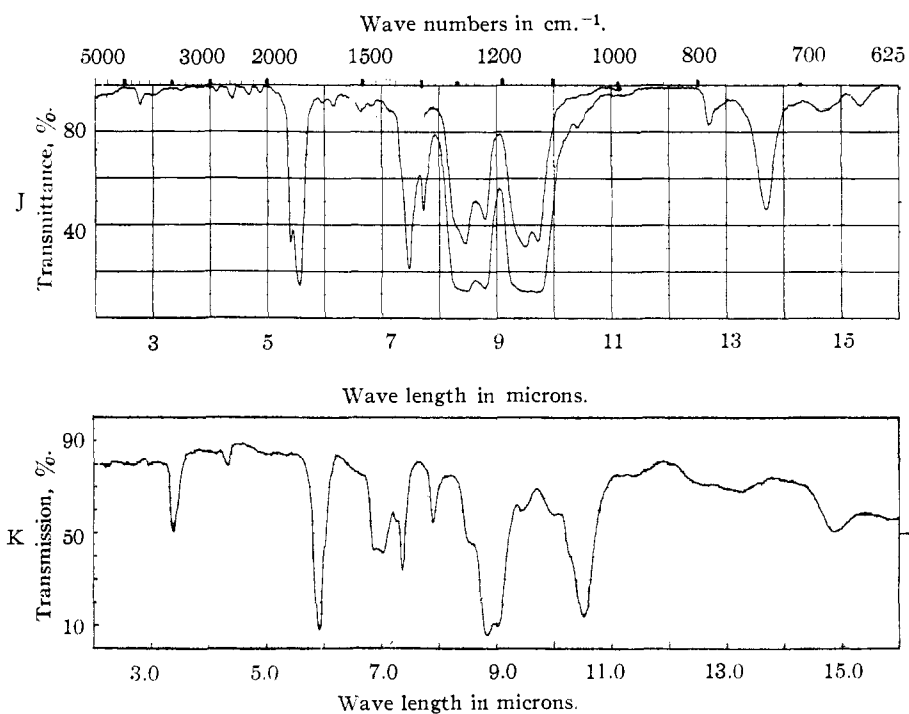
Fig. 4.—Infrared absorption spectra of perfluoroglutaric anhydride (J) and ethyl thioacetate (K).
