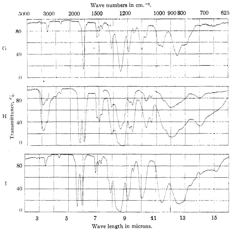
Fig. 3.—Infrared absorption spectra of diethyl dithiohexafluoroglutarate (G), monoethyl thiohexafluoroglutarate (H) and monoethyl thiohexafluoroglutaryl chloride (I).
